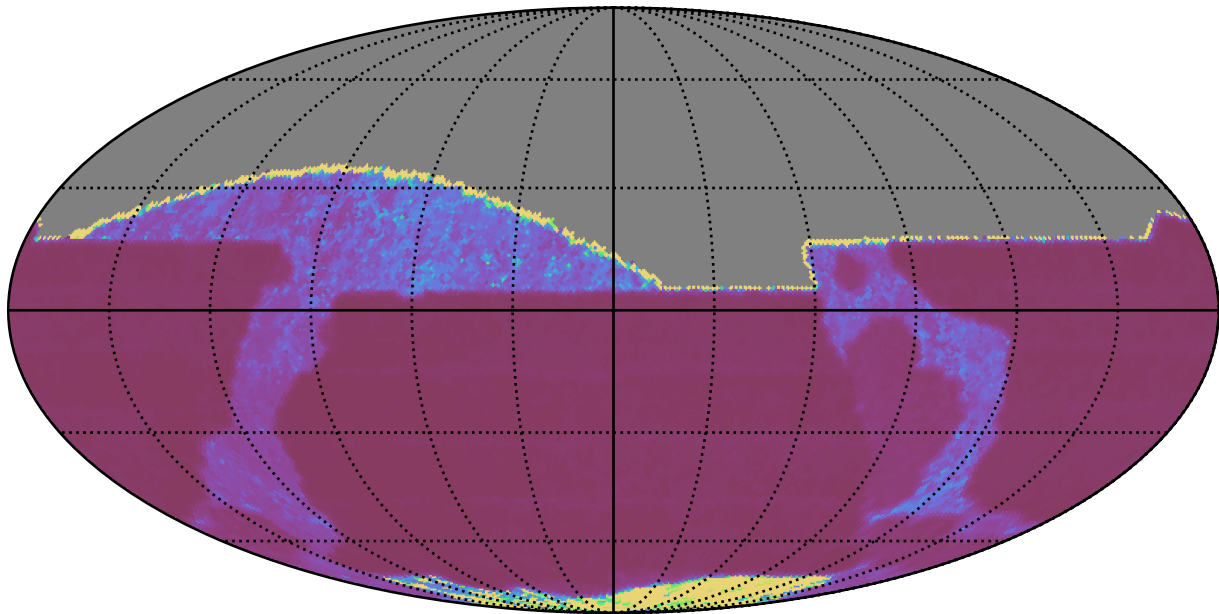
extra_ss_neo4_v3.4_10yrs All sky z band: Median Inter-Night Gap
