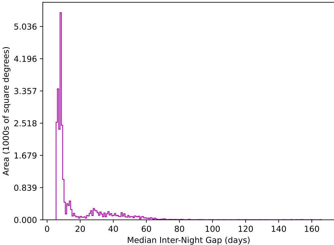
extra_ss_neo4_v3.4_10yrs All sky z band: Median Inter-Night Gap
