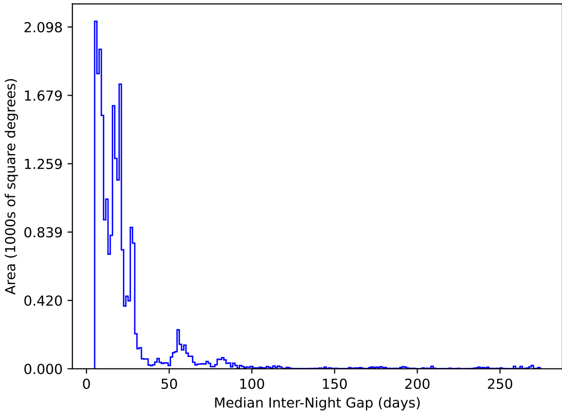
extra_ss_neo4_v3.4_10yrs All sky y band: Median Inter-Night Gap
