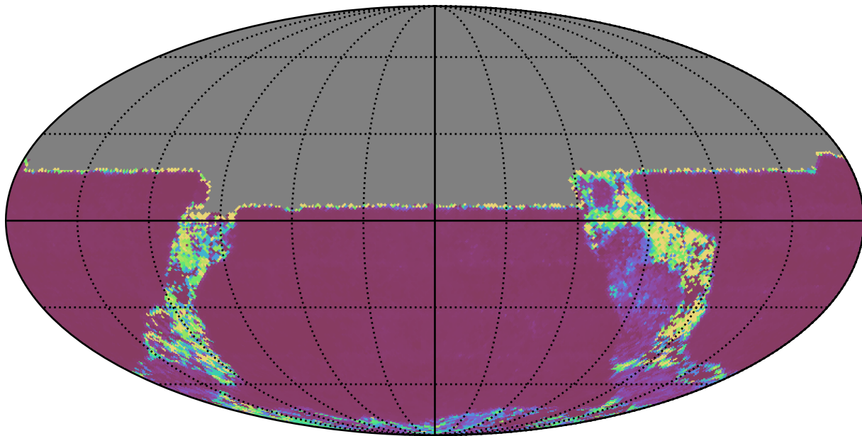
extra_ss_neo4_v3.4_10yrs All sky u band: Median Inter-Night Gap
