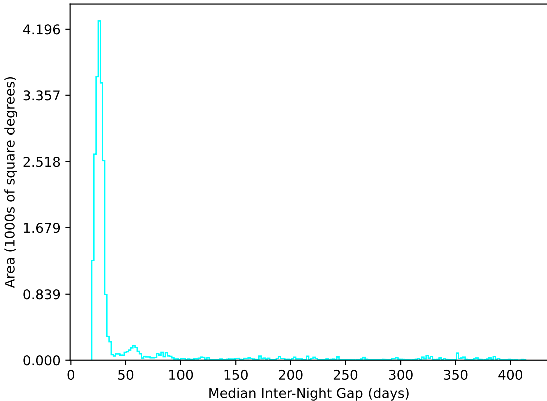
extra_ss_neo4_v3.4_10yrs All sky u band: Median Inter-Night Gap
