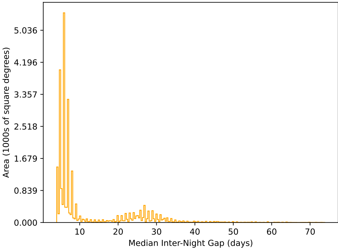
extra_ss_neo4_v3.4_10yrs All sky r band: Median Inter-Night Gap
