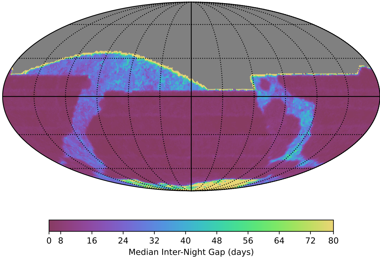
extra_ss_neo4_v3.4_10yrs All sky i band: Median Inter-Night Gap
