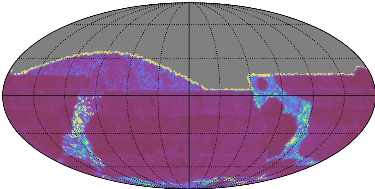
extra_ss_neo4_v3.4_10yrs All sky g band: Median Inter-Night Gap
