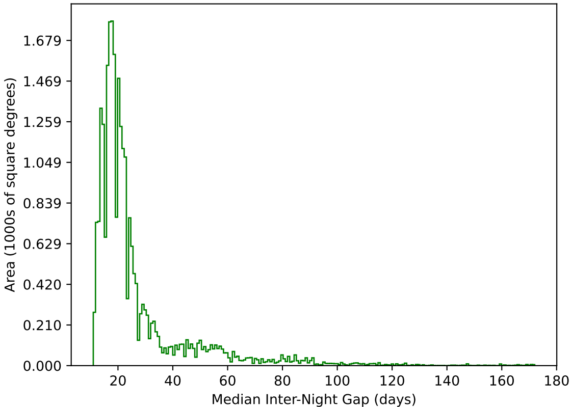
extra_ss_neo4_v3.4_10yrs All sky g band: Median Inter-Night Gap
