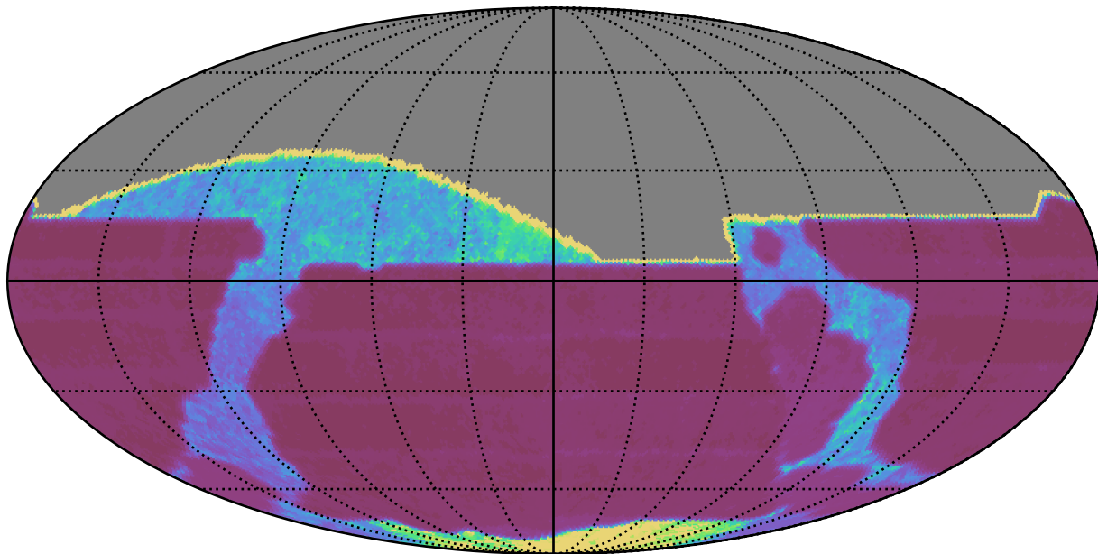
extra_ss_neo4_v3.4_10yrs All sky all bands: Median Inter-Night Gap
