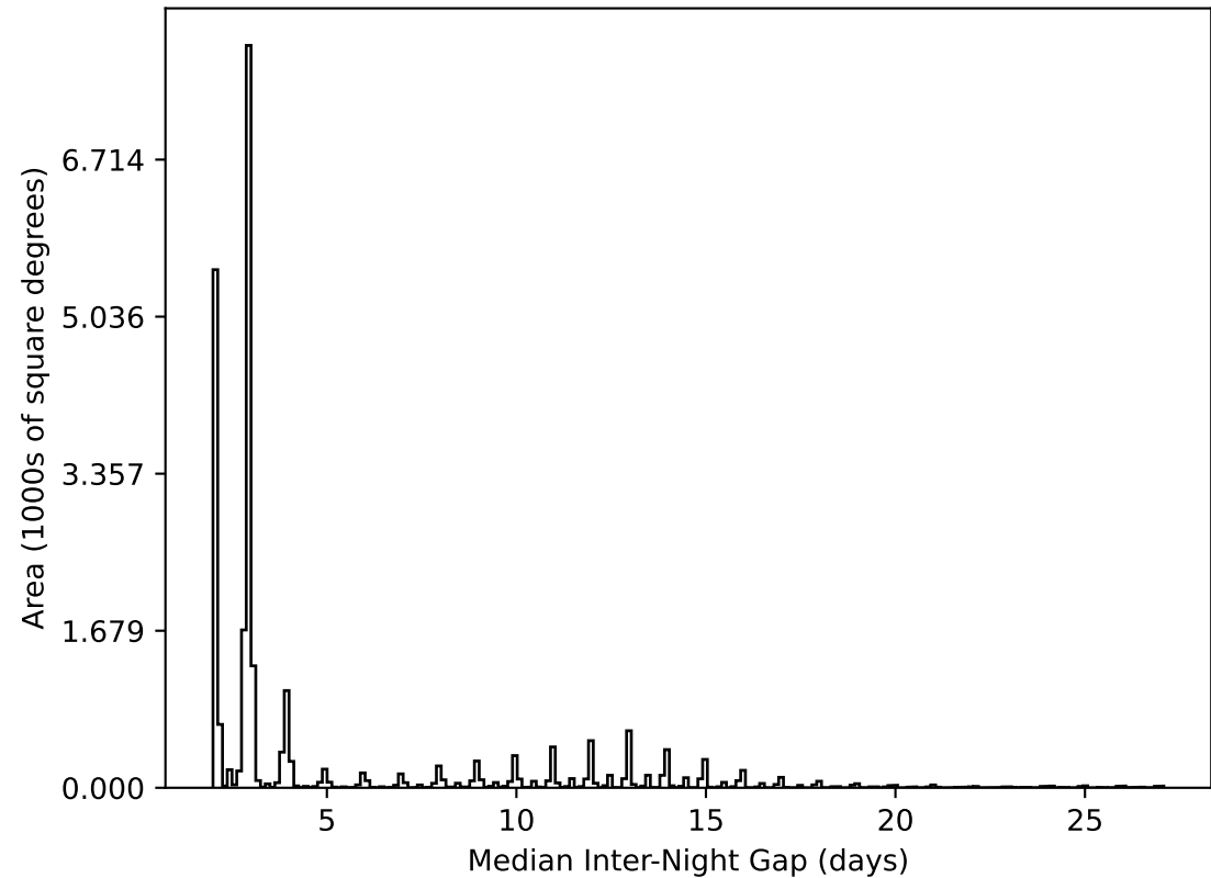
extra_ss_neo4_v3.4_10yrs All sky all bands: Median Inter-Night Gap
