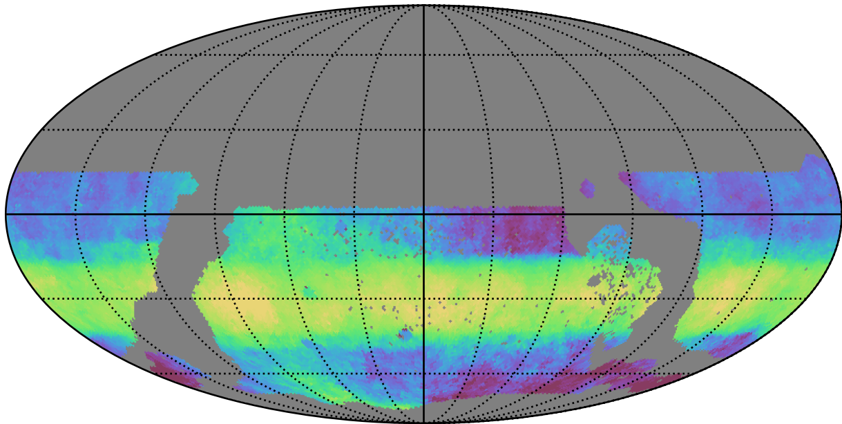
extra_ss_neo4_v3.4_10yrs WFD z band: Median HA
