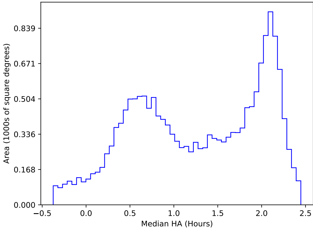
extra_ss_neo4_v3.4_10yrs WFD y band: Median HA
