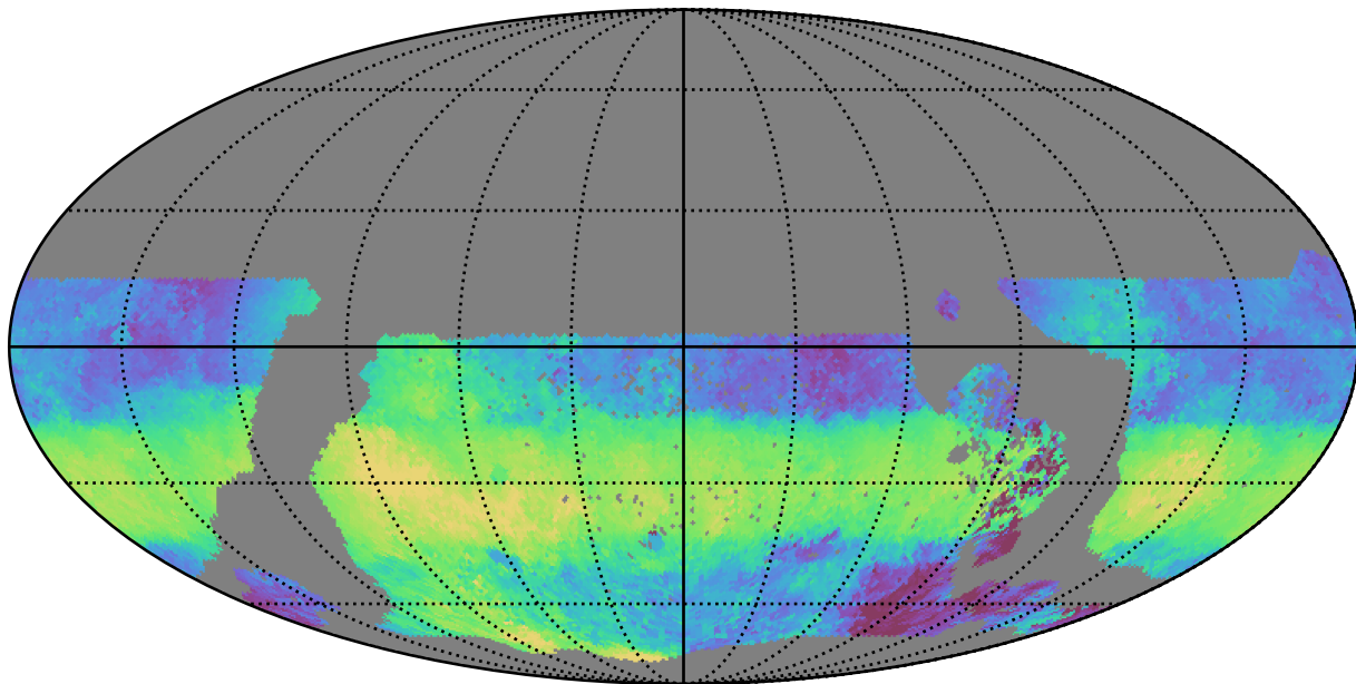
extra_ss_neo4_v3.4_10yrs WFD u band: Median HA
