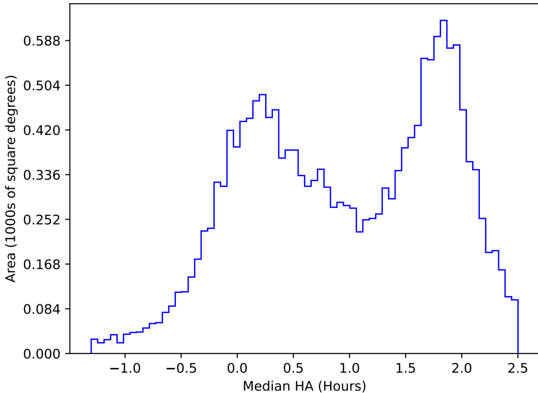
extra_ss_neo4_v3.4_10yrs WFD u band: Median HA
