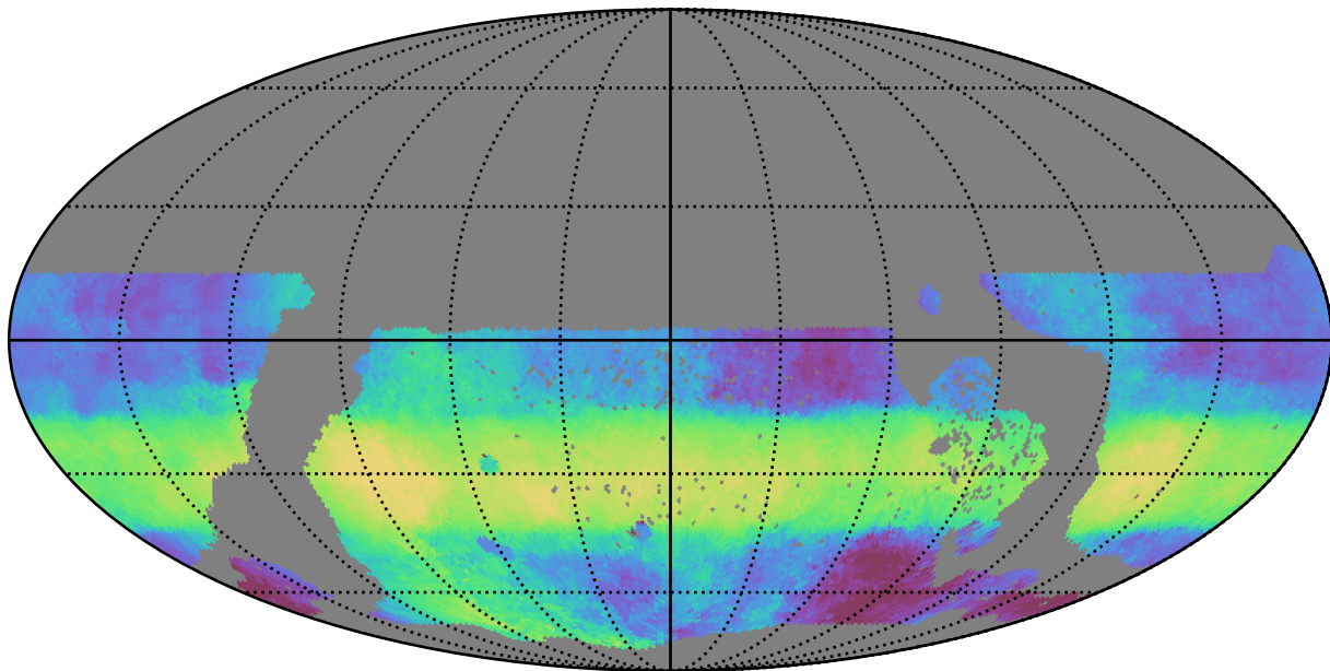
extra_ss_neo4_v3.4_10yrs WFD r band: Median HA
