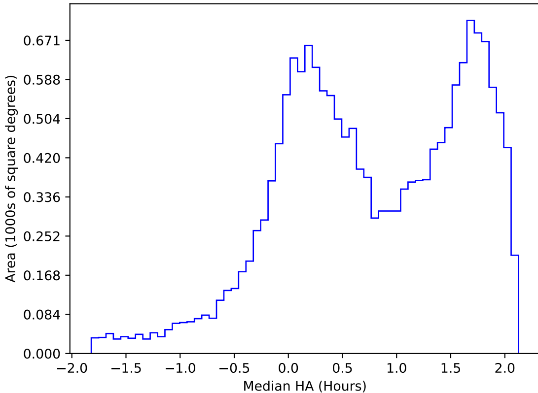
extra_ss_neo4_v3.4_10yrs WFD g band: Median HA
