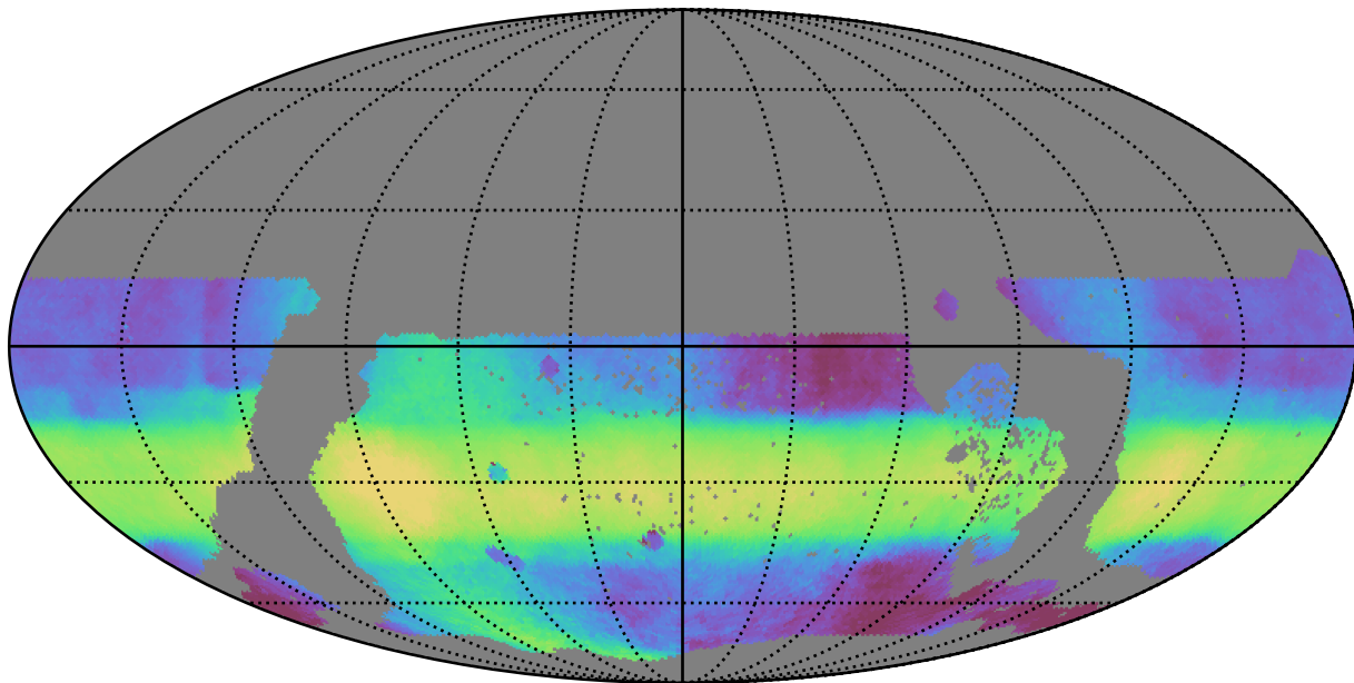
extra_ss_neo4_v3.4_10yrs WFD all bands: Median HA
