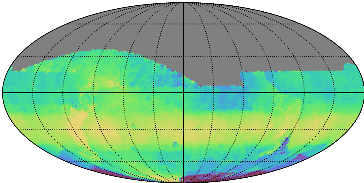
extra_ss_neo4_v3.4_10yrs All sky z band: Median HA
