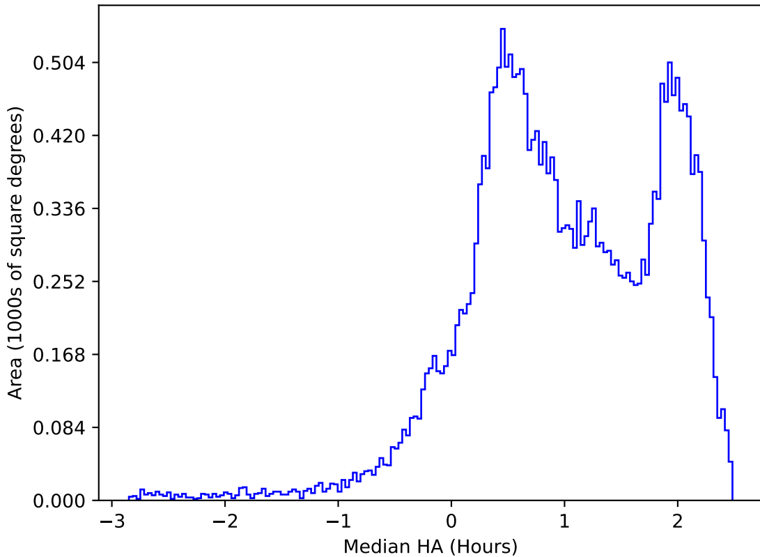
extra_ss_neo4_v3.4_10yrs All sky z band: Median HA
