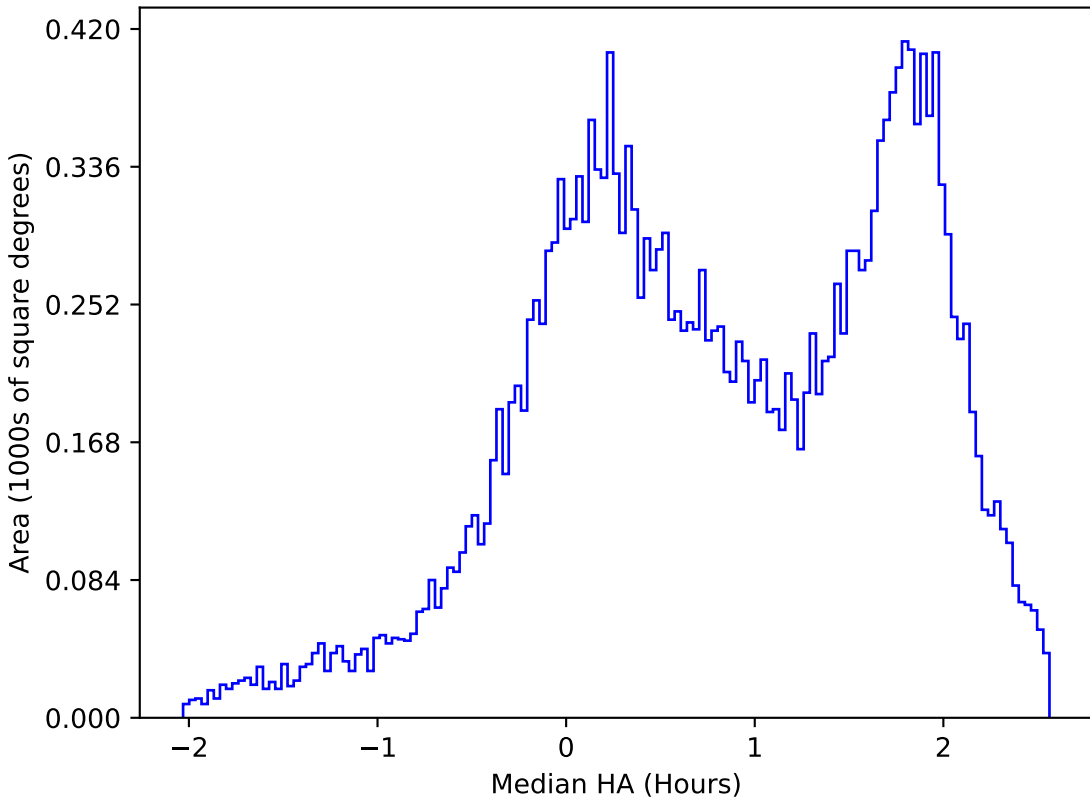
extra_ss_neo4_v3.4_10yrs All sky u band: Median HA
