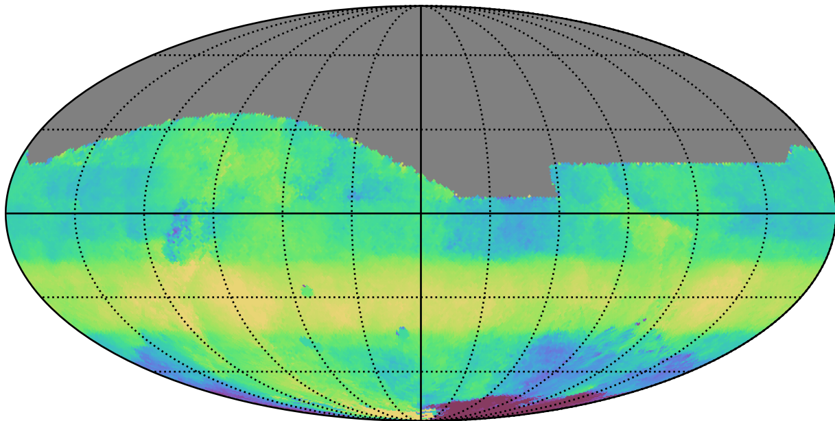
extra_ss_neo4_v3.4_10yrs All sky r band: Median HA
