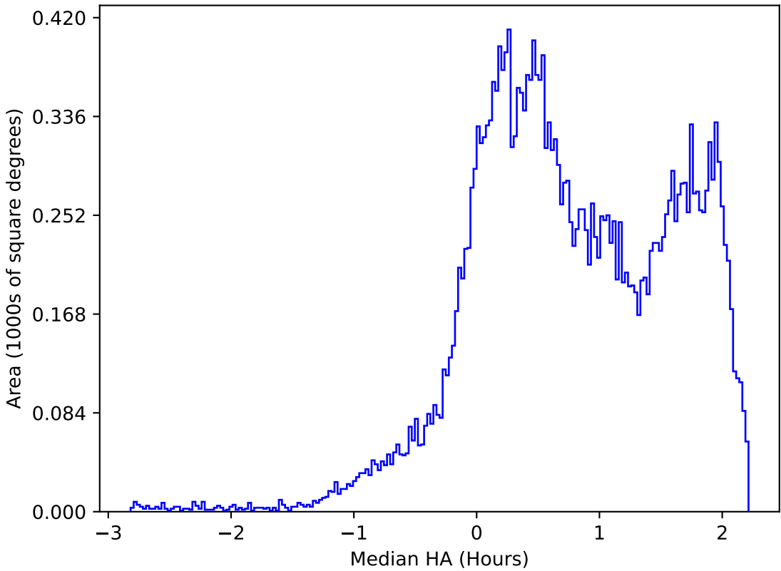
extra_ss_neo4_v3.4_10yrs All sky r band: Median HA
