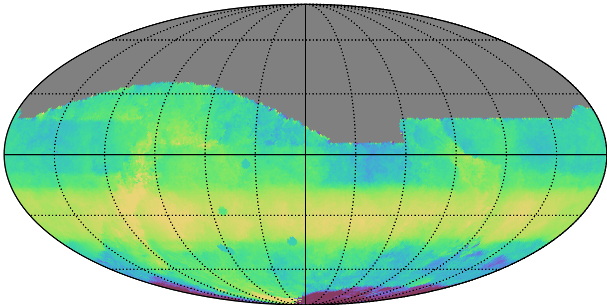
extra_ss_neo4_v3.4_10yrs All sky i band: Median HA
