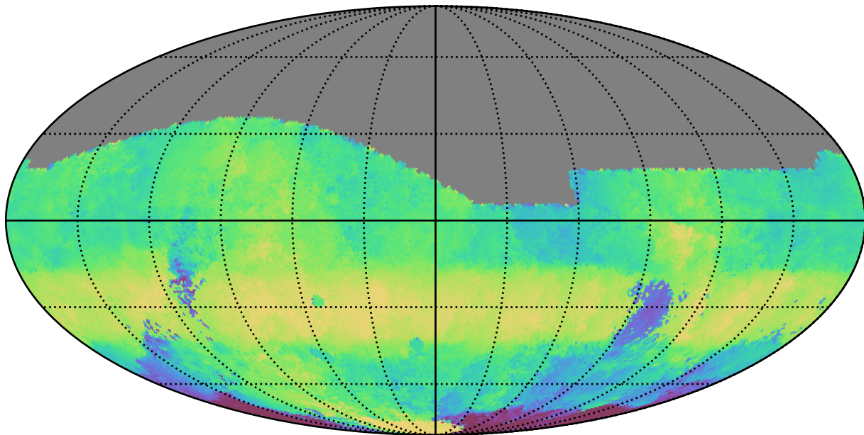
extra_ss_neo4_v3.4_10yrs All sky g band: Median HA
