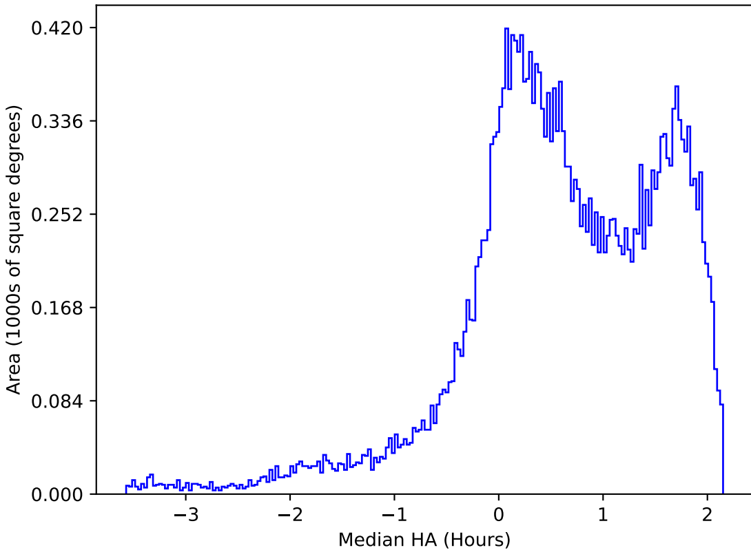
extra_ss_neo4_v3.4_10yrs All sky g band: Median HA
