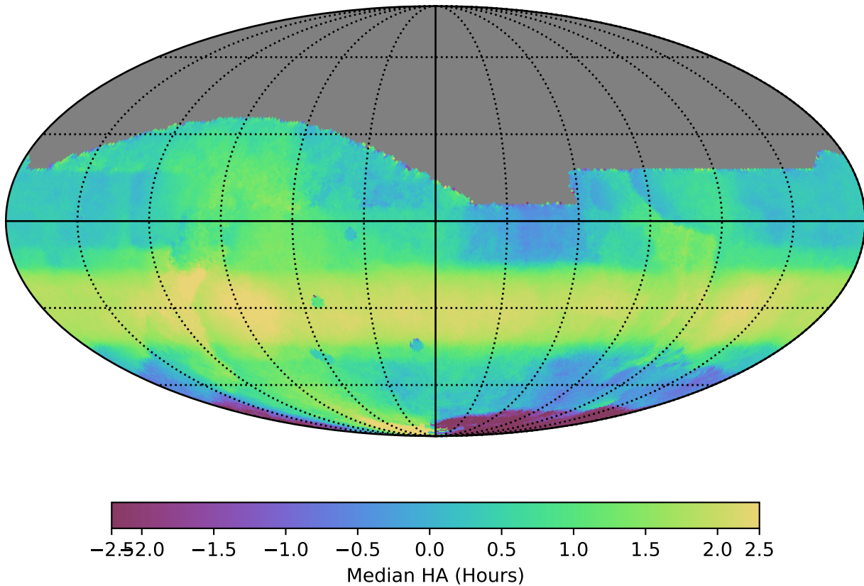
extra_ss_neo4_v3.4_10yrs All sky all bands: Median HA
