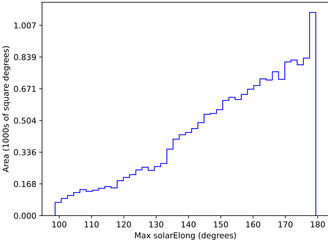
extra_ss_neo4_v3.4_10yrs WFD z band: Max solarElong
