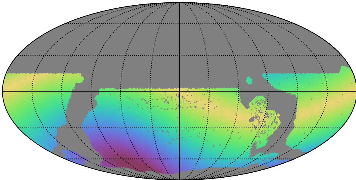
extra_ss_neo4_v3.4_10yrs WFD u band: Max solarElong
