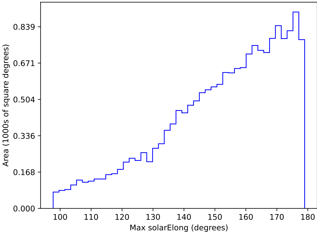
extra_ss_neo4_v3.4_10yrs WFD u band: Max solarElong
