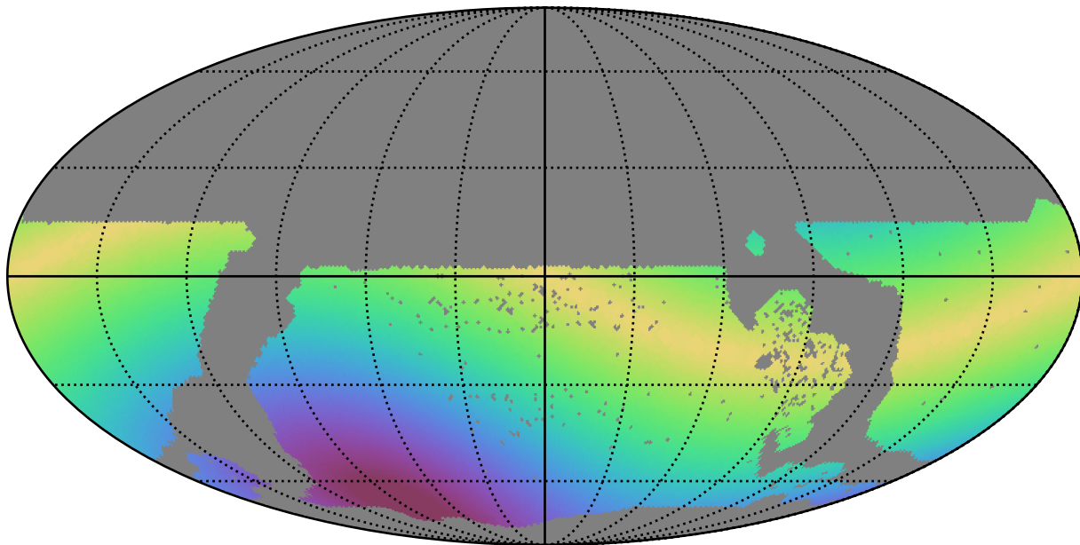
extra_ss_neo4_v3.4_10yrs WFD r band: Max solarElong
