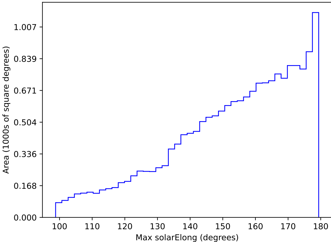
extra_ss_neo4_v3.4_10yrs WFD r band: Max solarElong
