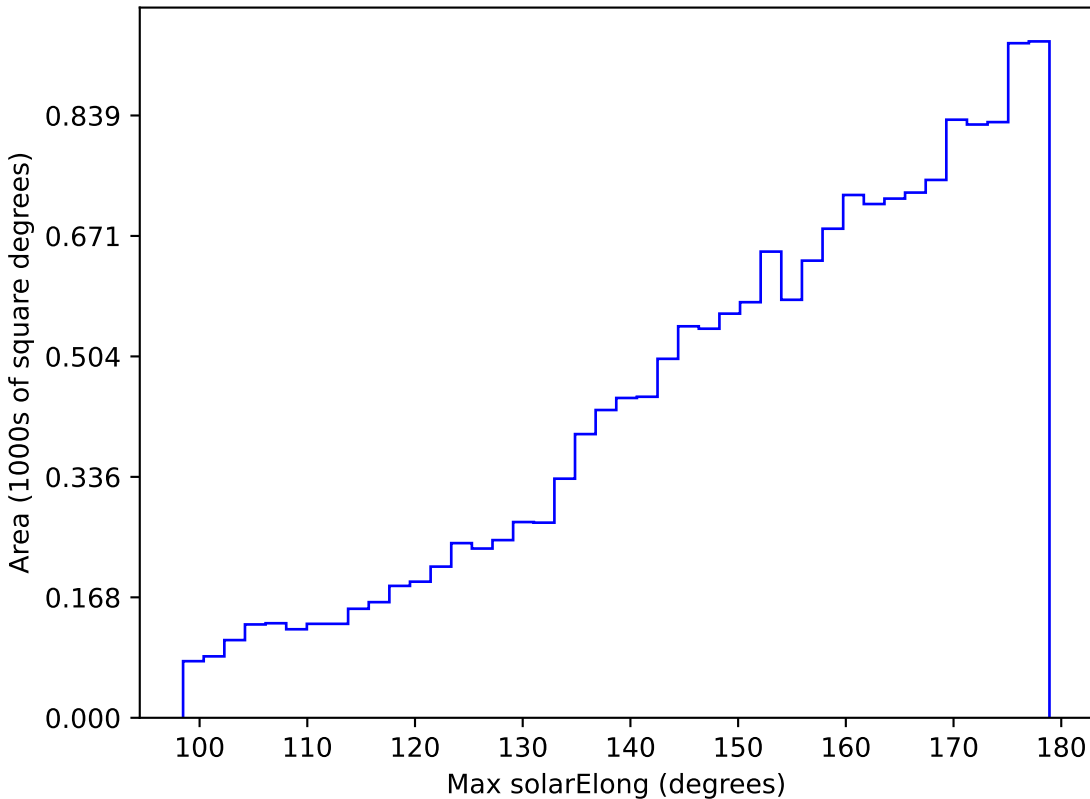
extra_ss_neo4_v3.4_10yrs WFD g band: Max solarElong
