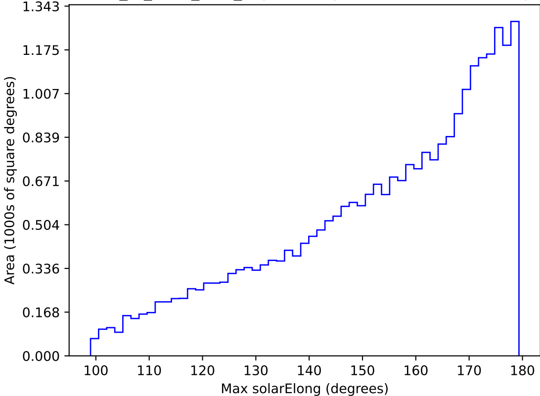
extra_ss_neo4_v3.4_10yrs All sky z band: Max solarElong
