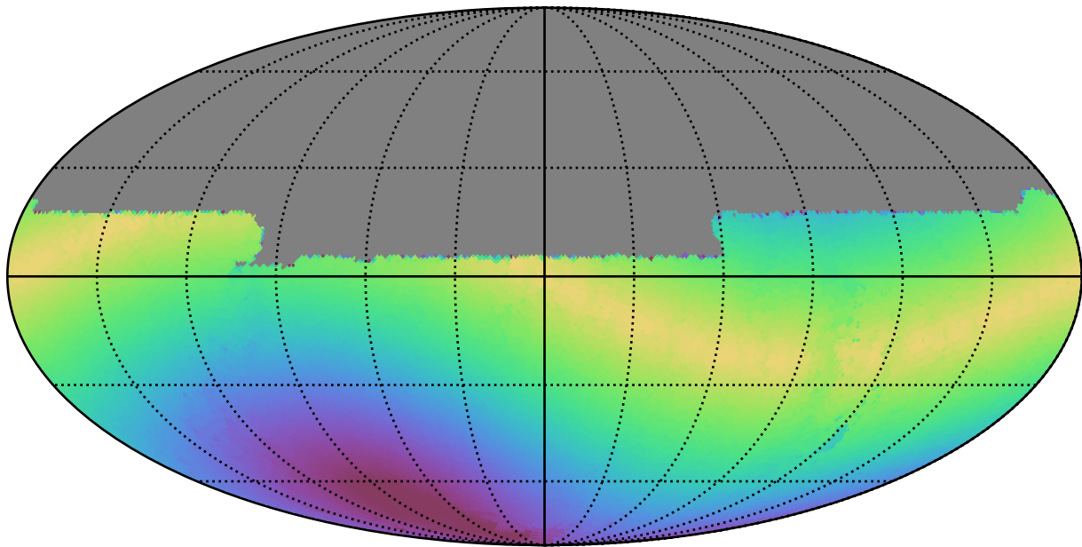
extra_ss_neo4_v3.4_10yrs All sky u band: Max solarElong
