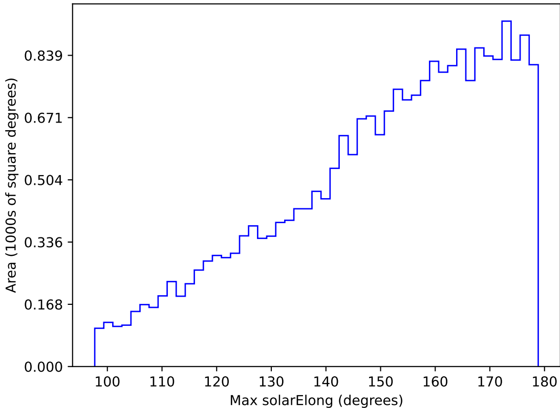
extra_ss_neo4_v3.4_10yrs All sky u band: Max solarElong
