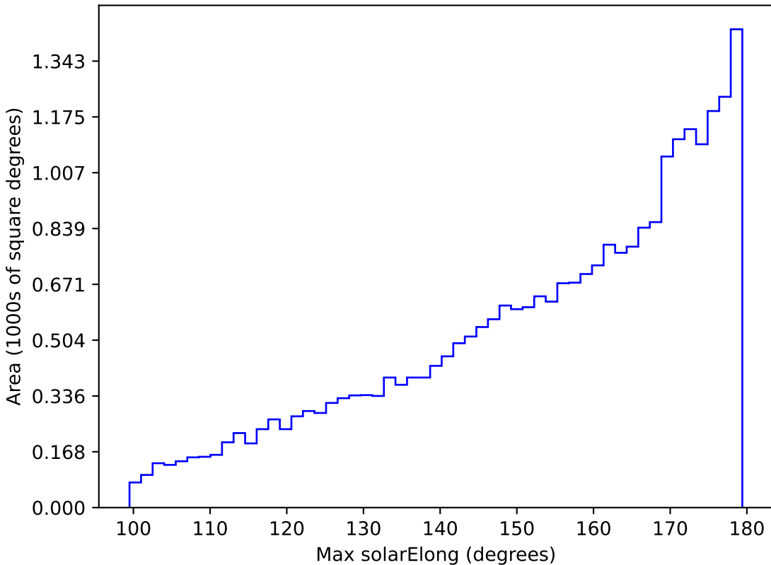
extra_ss_neo4_v3.4_10yrs All sky r band: Max solarElong
