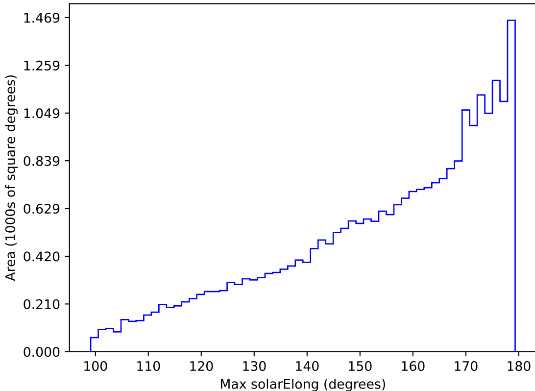
extra_ss_neo4_v3.4_10yrs All sky i band: Max solarElong
