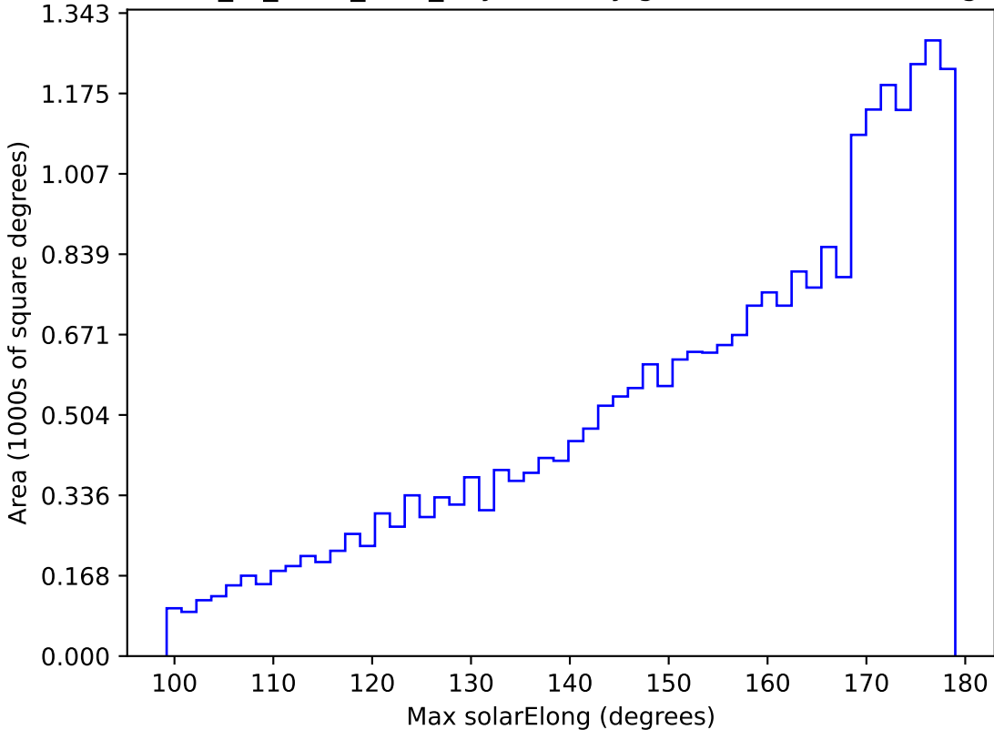
extra_ss_neo4_v3.4_10yrs All sky g band: Max solarElong
