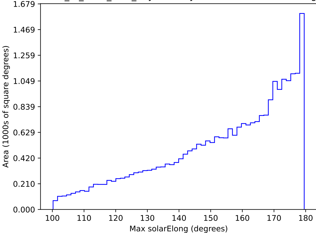
extra_ss_neo4_v3.4_10yrs All sky all bands: Max solarElong
