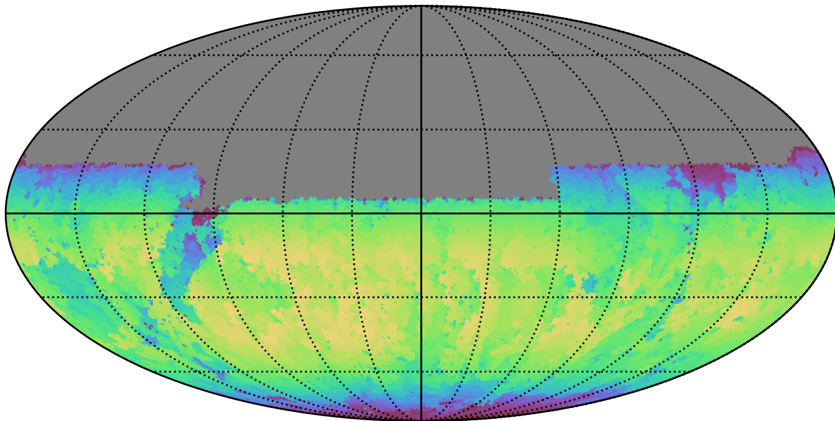
extra_ss_neo4_v3.4_10yrs Yr 1 y band: Max skyBrightness
