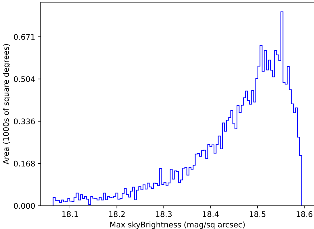
extra_ss_neo4_v3.4_10yrs Yr 1 y band: Max skyBrightness
