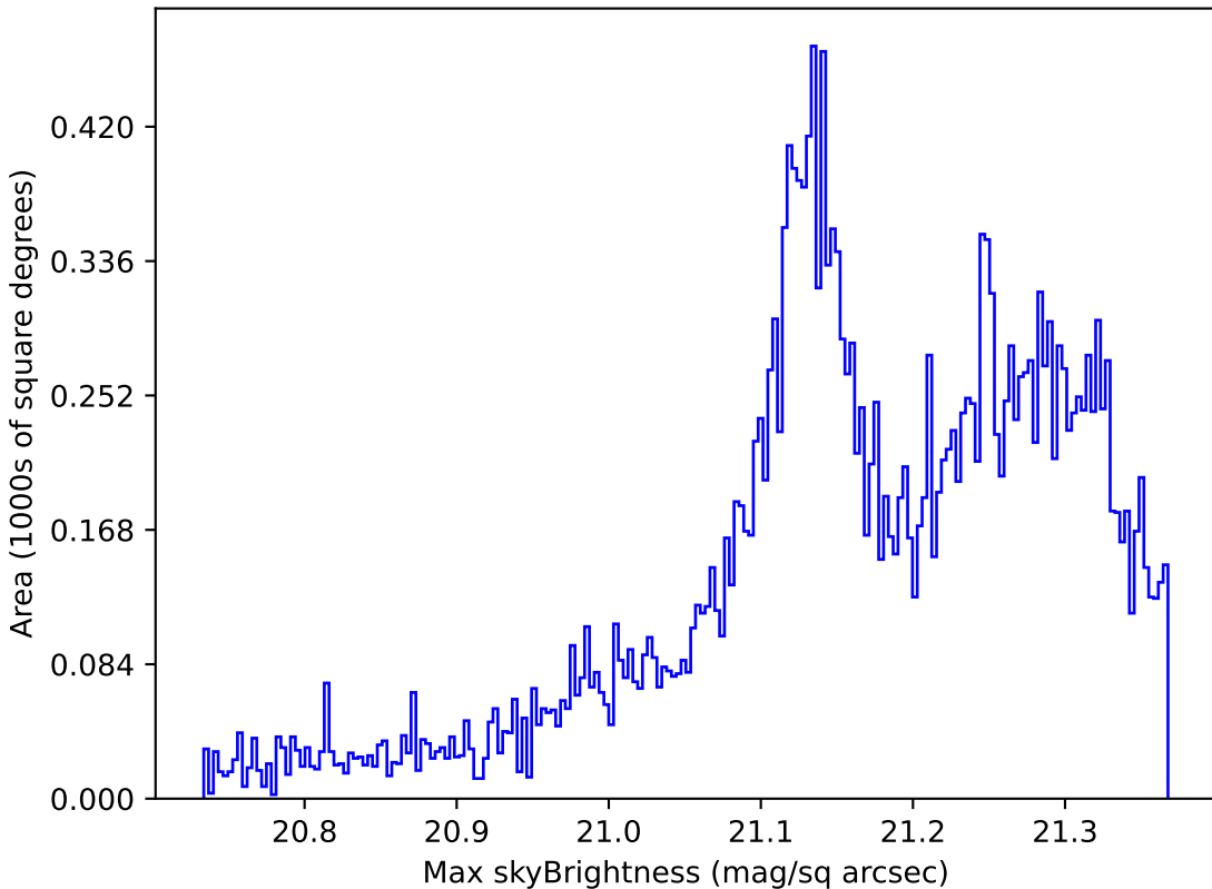
extra_ss_neo4_v3.4_10yrs Yr 1 r band: Max skyBrightness
