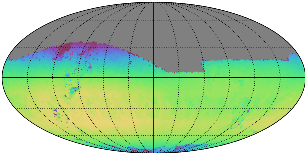
extra_ss_neo4_v3.4_10yrs Yr1 i band: Max skyBrightness
