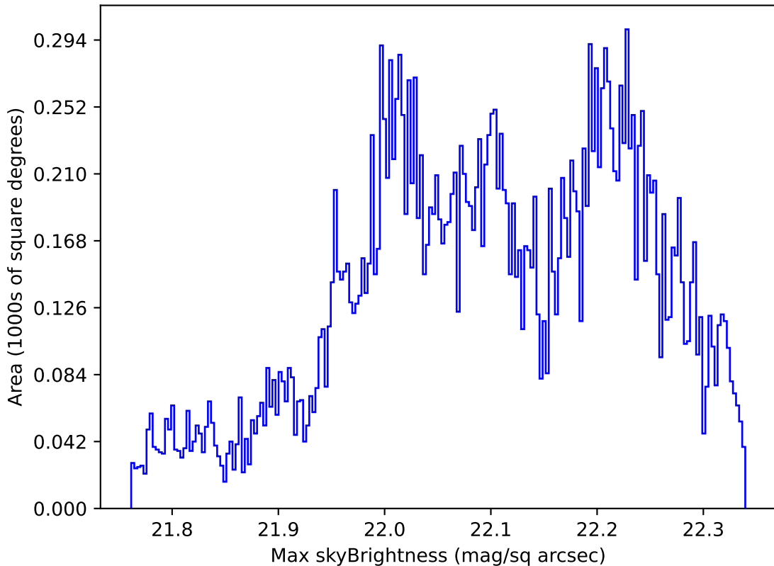
extra_ss_neo4_v3.4_10yrs Yr 1 g band: Max skyBrightness
