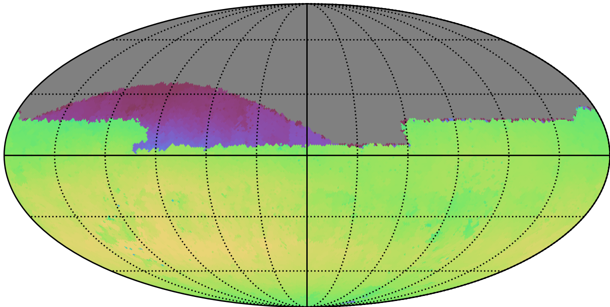
extra_ss_neo4_v3.4_10yrs Yr 1 all bands: Max skyBrightness
