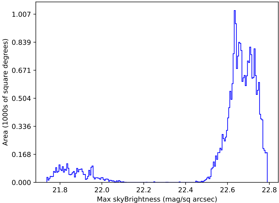
extra_ss_neo4_v3.4_10yrs Yr 1 all bands: Max skyBrightness
