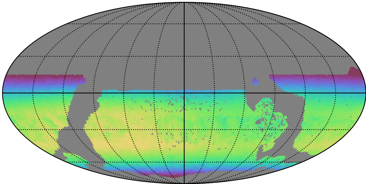
extra_ss_neo4_v3.4_10yrs WFD z band: Max skyBrightness
