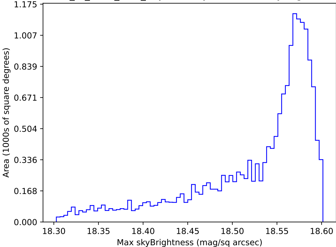
extra_ss_neo4_v3.4_10yrs WFD y band: Max skyBrightness
