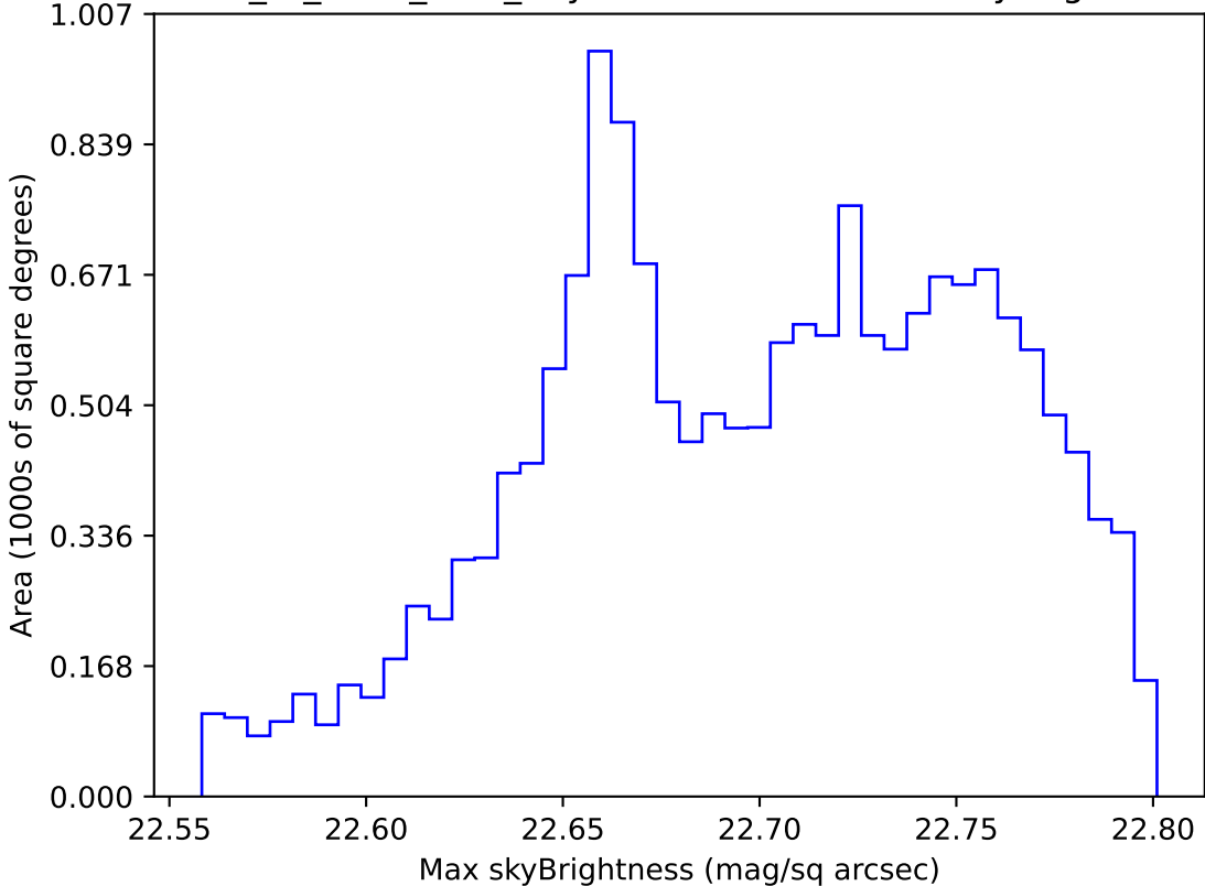
extra_ss_neo4_v3.4_10yrs WFD u band: Max skyBrightness
